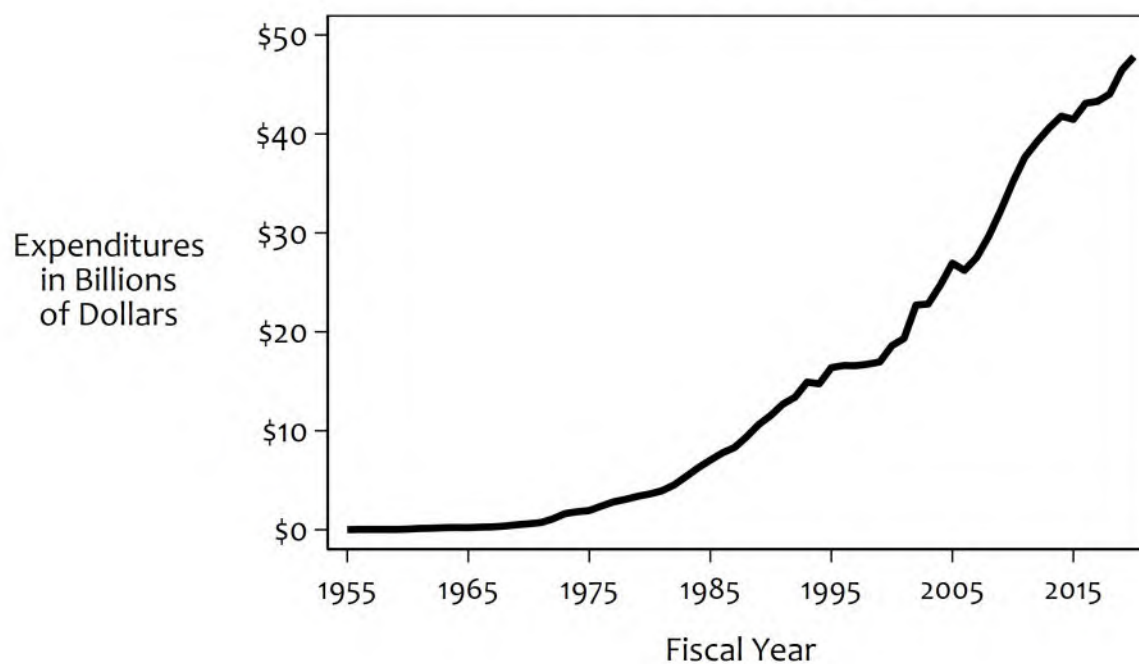
Figure 1: Public Health Expenditures for Ontario, 1954/55 through 2019/20
