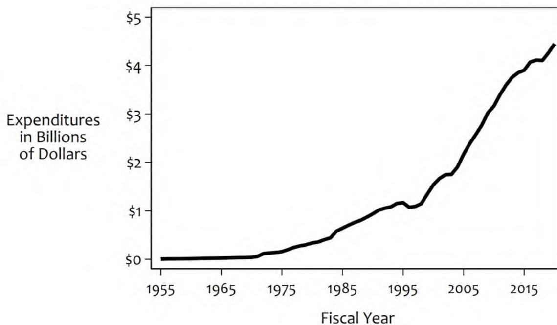
Figure 1: Public Health Expenditures for Nova Scotia, 1954/55 through 2019/20
