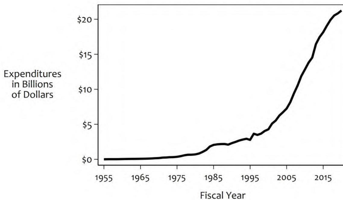
Figure 1: Public Health Expenditures for Alberta, 1954/55 through 2019/20
