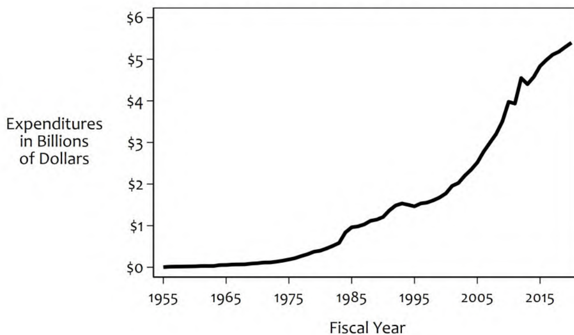
Figure 1: Public Health Expenditures for Saskatchewan, 1954/55 through 2019/20
