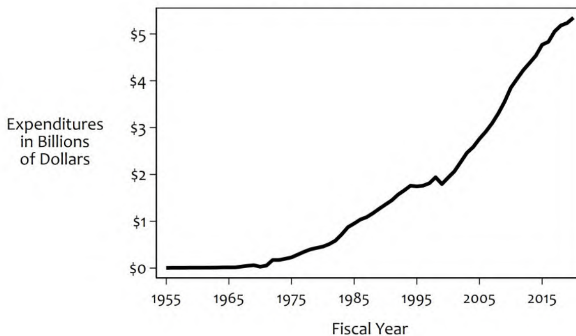
Figure 1: Public Health Expenditures for Manitoba, 1954/55 through 2019/20
