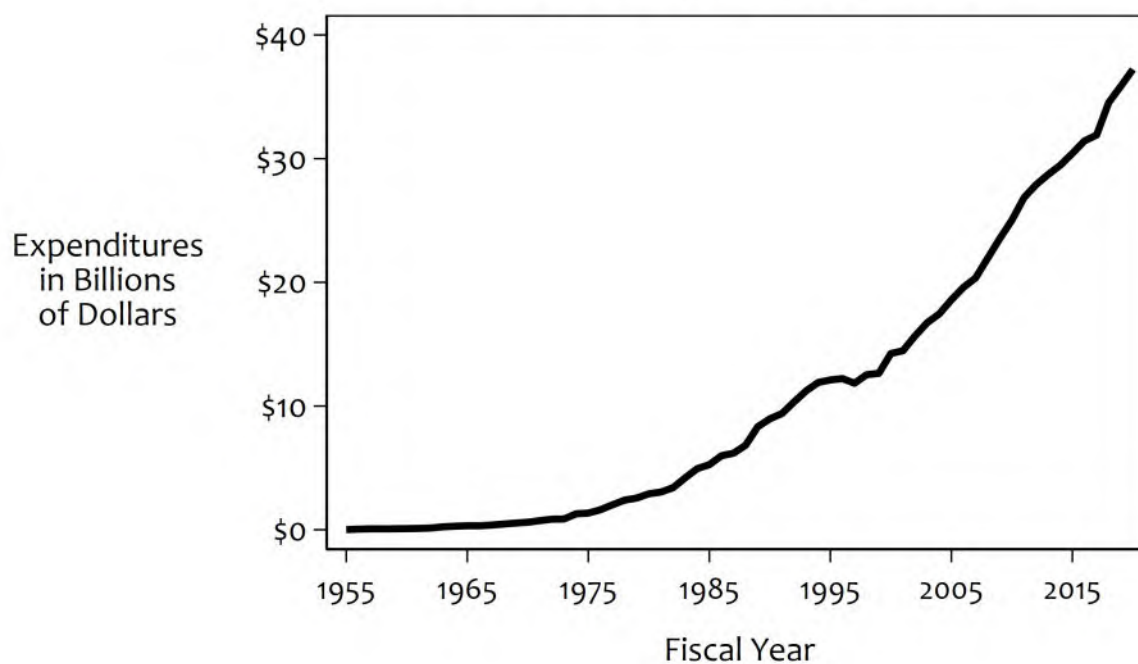
Figure 1: Public Health Expenditures for Quebec, 1954/55 through 2019/20
