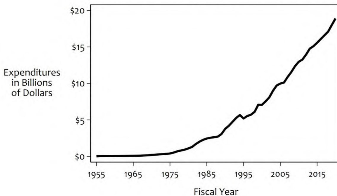
Figure 1: Public Health Expenditures for British Columbia, 1954/55 through 2019/20
